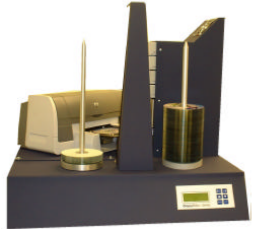
The CopyDisc4S -Opti Automatic CD-R/DVD-R Duplicator and Ink-jet Printer
